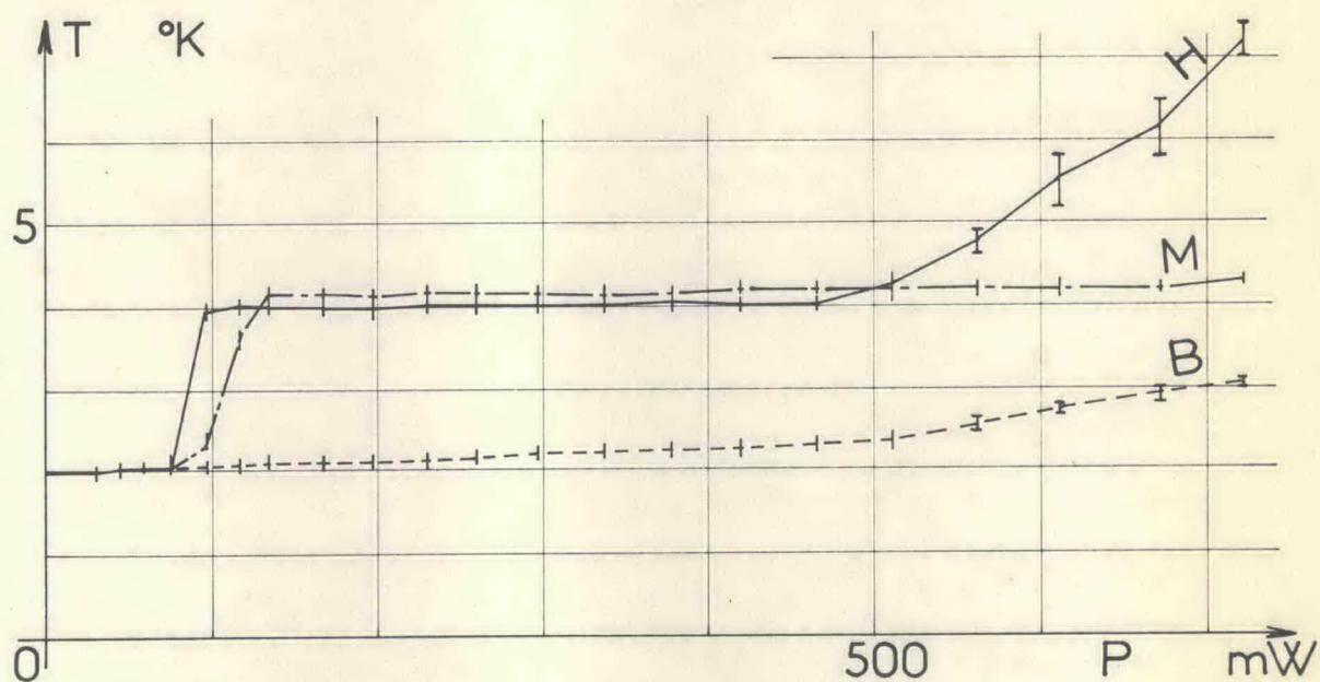
FIG.12 : Superfluid helium T = 2 K ; p = 1 atm
